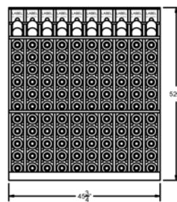
ELEVATION -E-
